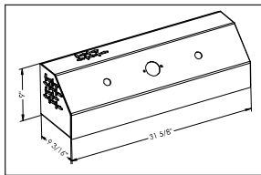
3533 - Diamond Plate with 2" Round Light Holes
