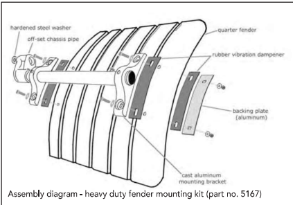
Assembly diagram - heavy duty fender mounting kit (part no. 5167)
