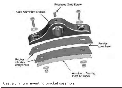
Cast aluminum mounting bracket assembly.
