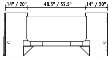
FRONT Configuration
